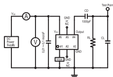
CD : DC-Cut capacitance RL : 10kΩ ± 10% CL : 10pF ± 10% including fixture and probe capacitance
