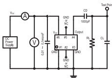
CD : DC-Cut capacitance RL : 10kΩ ± 10% CL : 10pF ± 10% including fixture and probe capacitance
